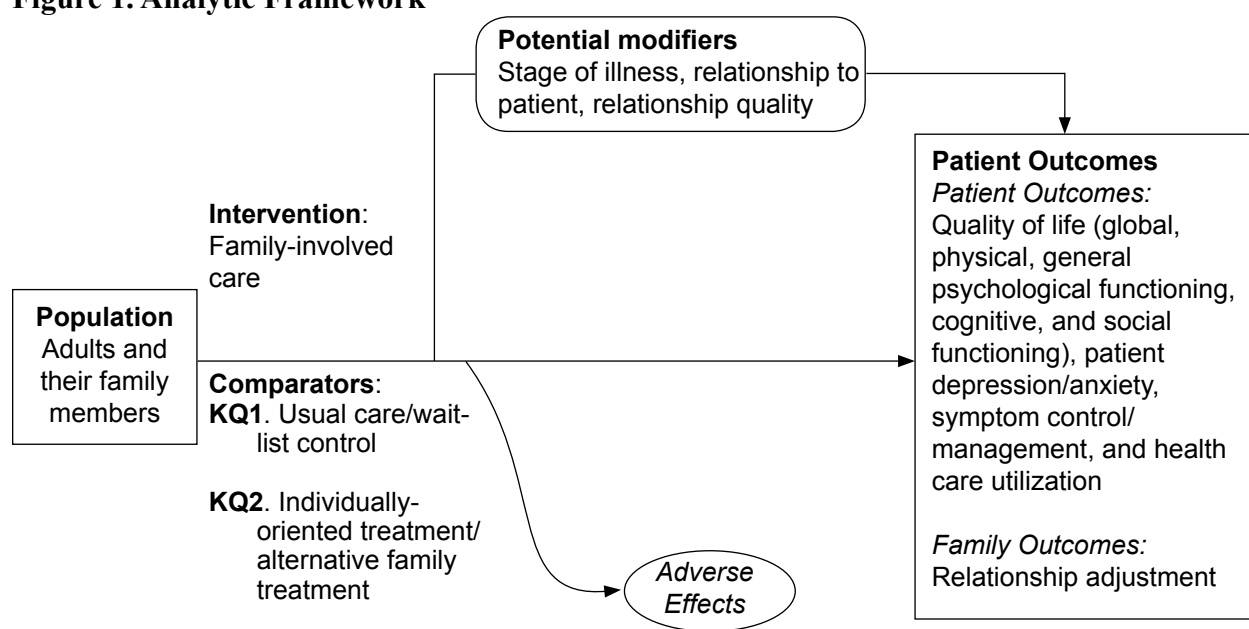
Figure 1. Analytic Framework
