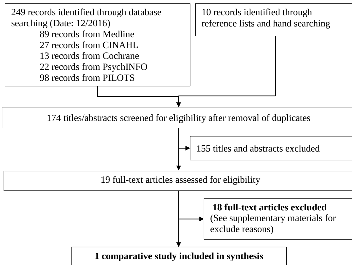
Figure 1: Literature Flowchart
